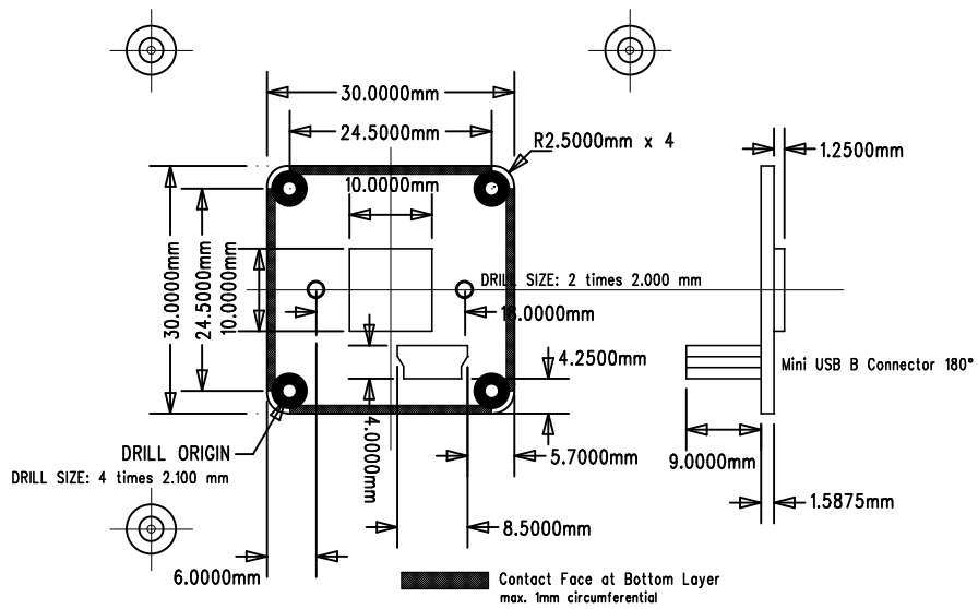
DRILL DRAWING
